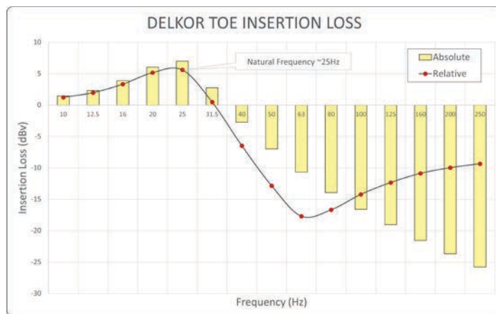
Relative Insertion Loss Reference Track – 150kN/mm
